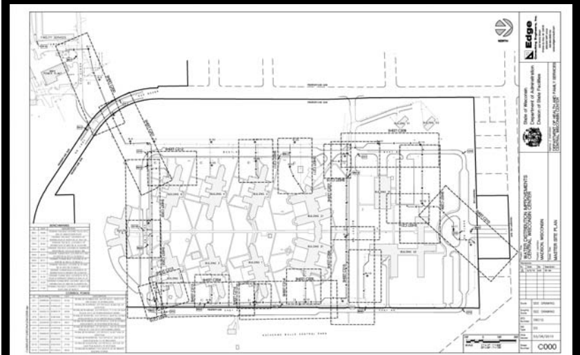
Overall Utility Plan
